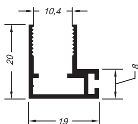
Transpasse 10mm
