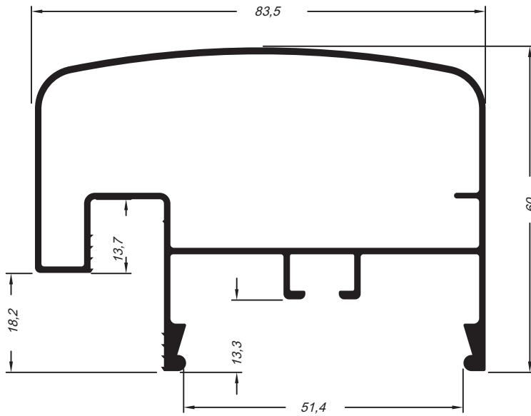
MK-83 Corrimão sacada retangular 1,163 Kg/m
