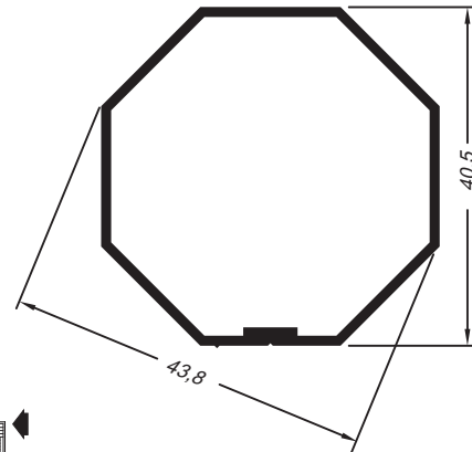
Tubo octagonal
