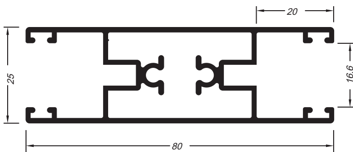
Guia lateral palheta
