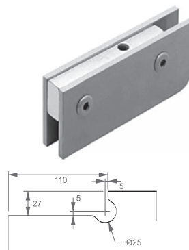
1101A /// Dobradiça superior
